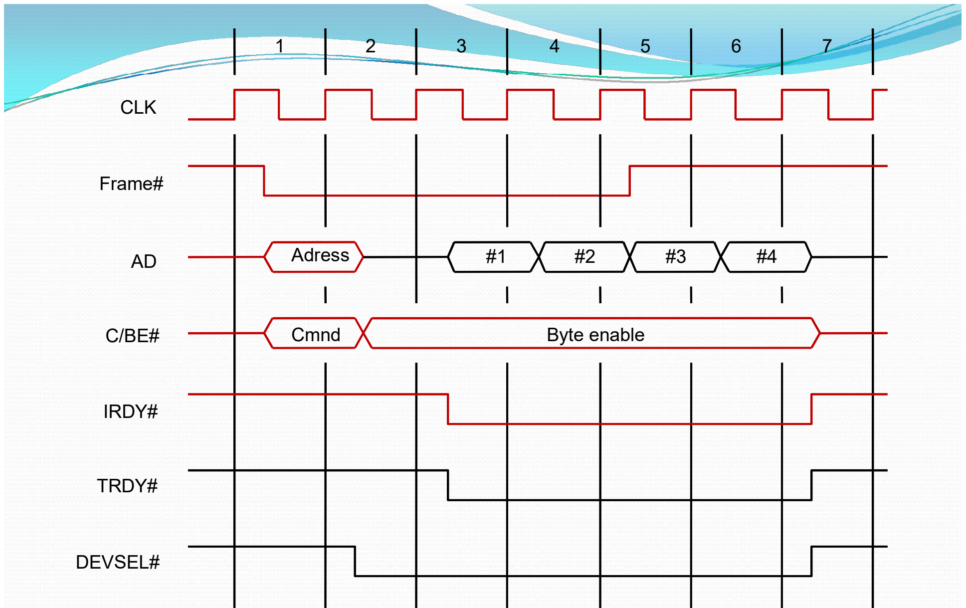
A read operation on the PCI bus
